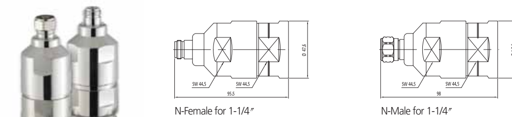
Connector N Type for 1-1/4" LHF & HFC
