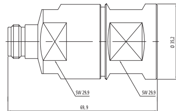
N-Female for 7/8"
