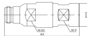
N-Female for 1/2"
