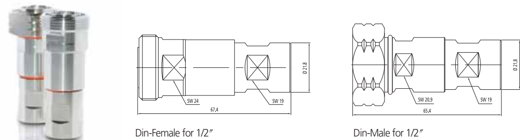
Connector Din Type for 1/2" LHF & HFC & HFSC
