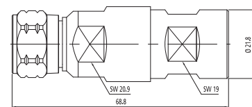
N-Male for 1/2"
