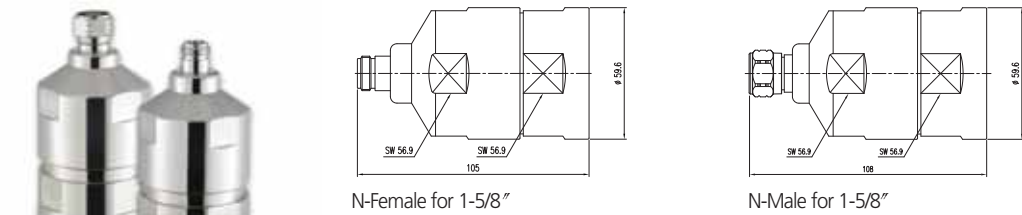
Connector N Type for 1-5/8" LHF & HFAC & HFC
