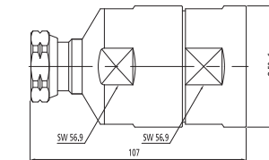
Din-Male for 1-5/8"
