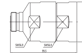
Din-Female for 1-5/8"
