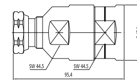
Din-Male for 1-1/4"
