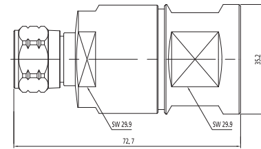
N-Male for 7/8"
