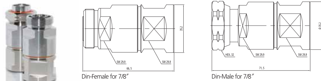
Connector Din Type for 7/8" LHF & HFAC & HFC
